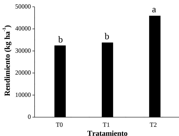
Figure 4. Total yield of potato variety Desiree established in Andisol in the Region of La Araucania. Different letters Indicate significant Differences bars ACCORDING TO Tukey's test ( p \leq 0.05 ).
