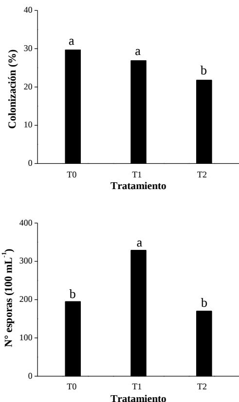
Figure 2. Parameters fungal roots and rhizosphere of potato variety Andisol established in the Region of La Araucania Desiree: A) Percentage AMF colonization and B) Number of spores HMA. Bars followed by different letters are significantly different according to Tukey test ( p \leq 0.05 ).
